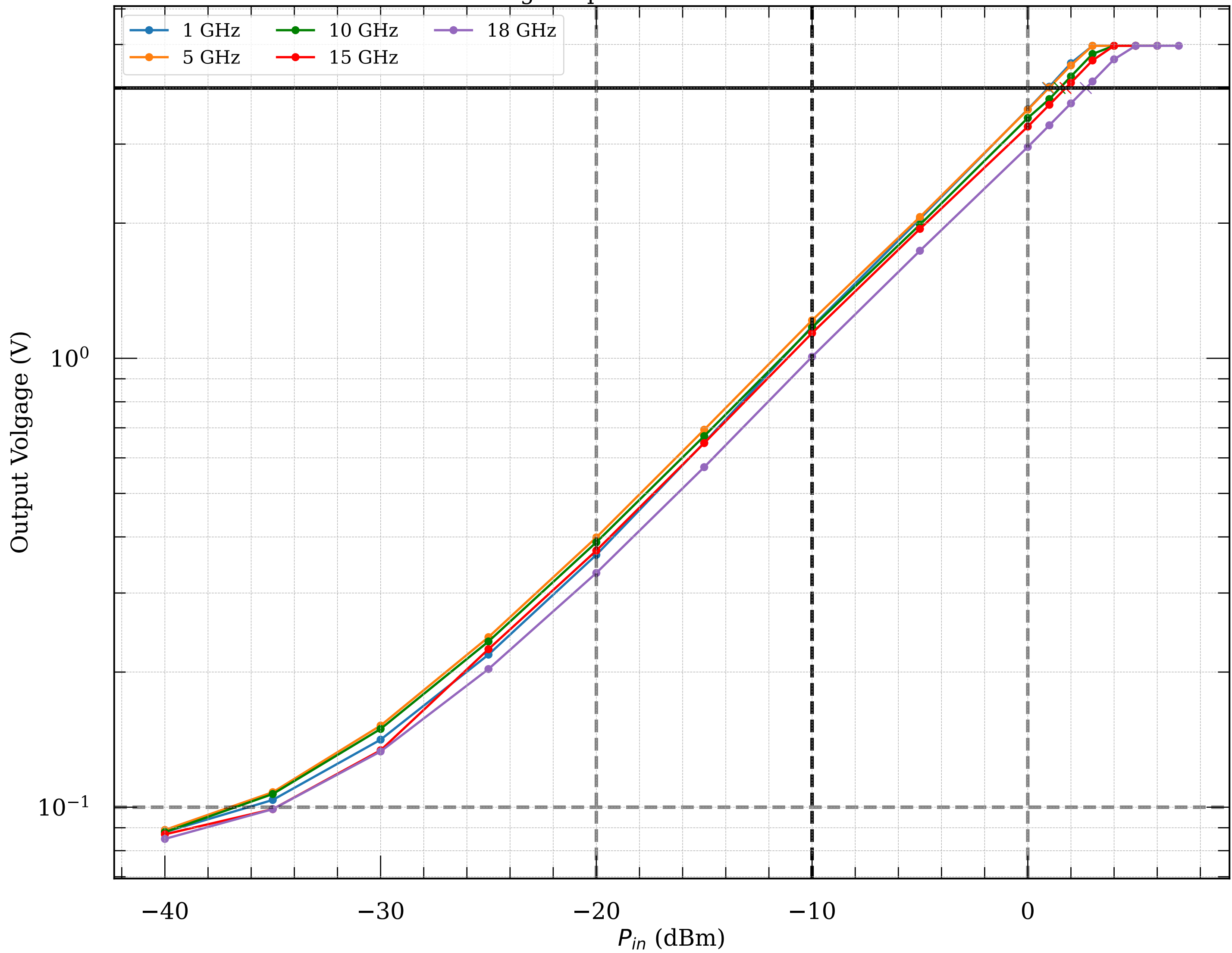
Measured voltage-to-power curve of detector module071
